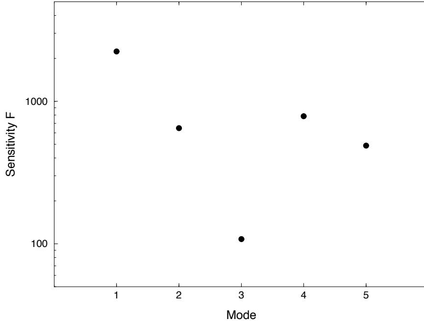
Figure 4.5: Detection sensitivity for a hypothetical ^{26}\text{Mg}+\text{p} resonance at E_R = 0.23 MeV, decaying to the ground state through an intermediate level at E_x = 1 MeV via a two- \gamma -ray cascade. The vertical axis displays the factor F = (1 + \sqrt{\Delta E_\gamma \overline{B}}) / \eta_\gamma^{G_e, P} of Eq. 4.5. On the horizontal axis, the numbers 1, 2, 3, 4 and 5 indicate the mode of operation corresponding to the spectra shown in Figs. 4.2(a), 4.2(b), 4.2(c), 4.4(a) and 4.4(b), respectively.
