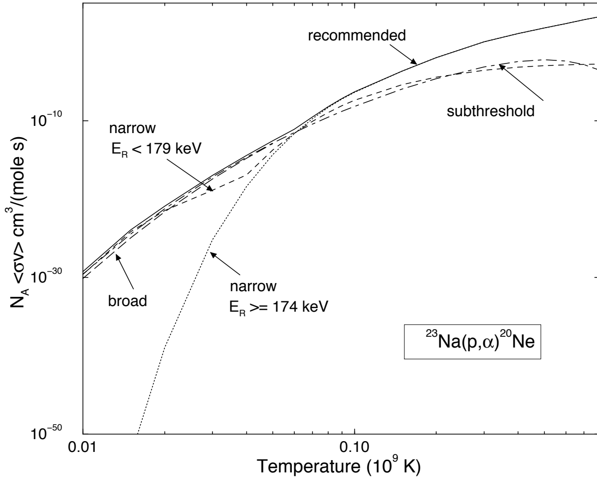
Figure 7.1: Contributions to the ^{23}\text{Na}(p,\alpha)^{20}\text{Ne} reaction rate from narrow, broad, and subthreshold resonances. Total recommended rate is given by the solid line.
