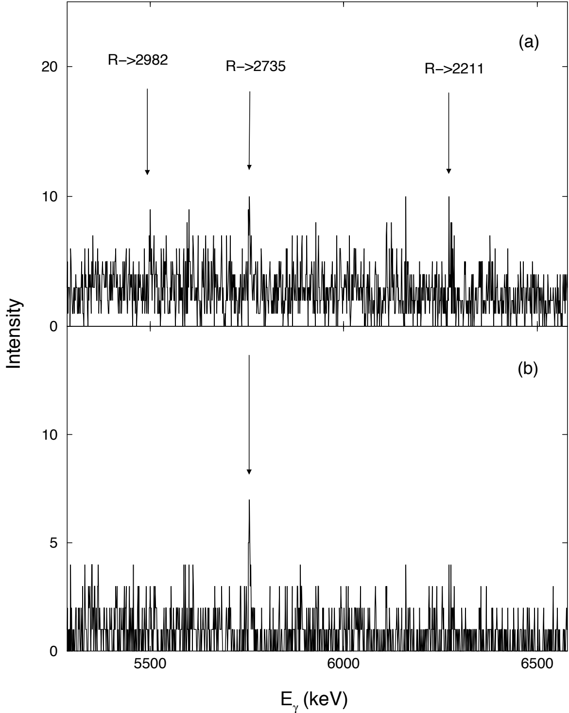
Figure 4.4: Germanium detector spectra for the E_R = 227 keV resonance in ^{26}\text{Mg}+p in the region E_\gamma^{Ge} = 5400\text{--}6500 keV, measured with a proton beam intensity of I_p \approx 1.5\mu\text{A} and a running time of 10 hours: (a) Singles spectrum without lead shield. Very weak \gamma -ray lines are observed corresponding to the strongest primary transitions in ^{27}\text{Al} ; (b) Coincidence spectrum (without lead shield) obtained with the condition 0.25\text{ MeV} < (E_\gamma^{Ge} + E_\gamma^{NaI}) < 9.0\text{ MeV} . The primary transition to the fourth excited state in ^{27}\text{Al} is clearly seen.
